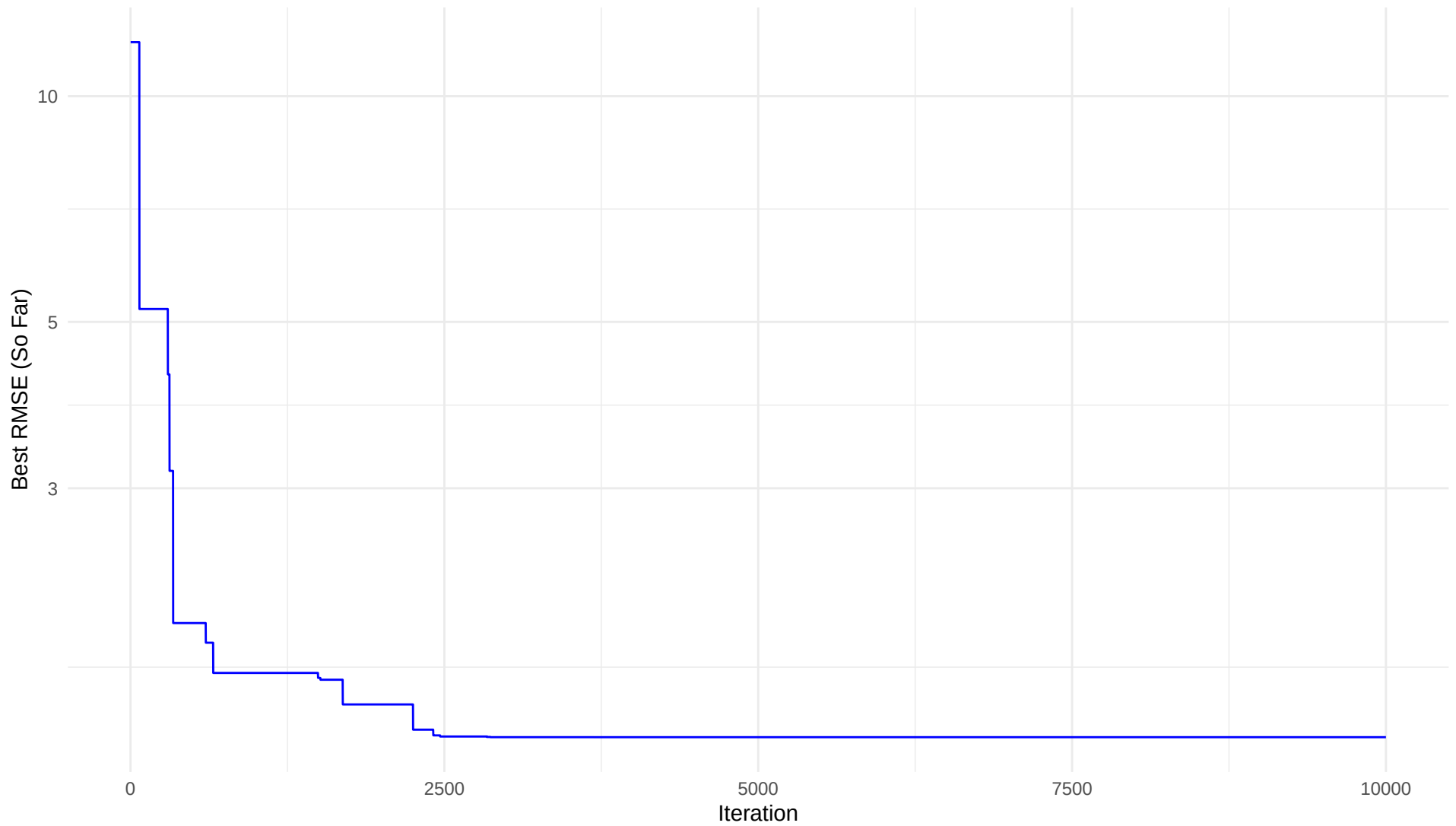
Best RMSE Convergence: Location stjoseph Fold 5
