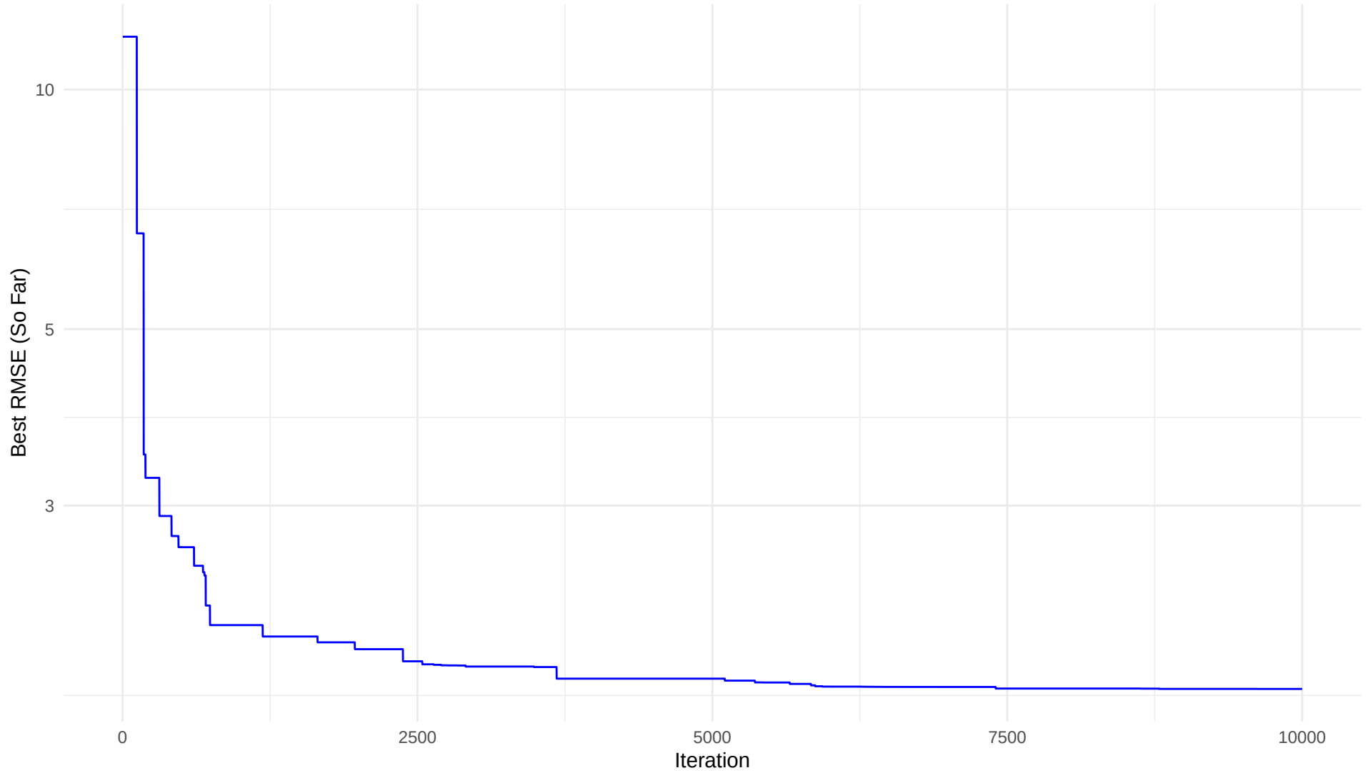
Best RMSE Convergence: Location humber Fold 5
