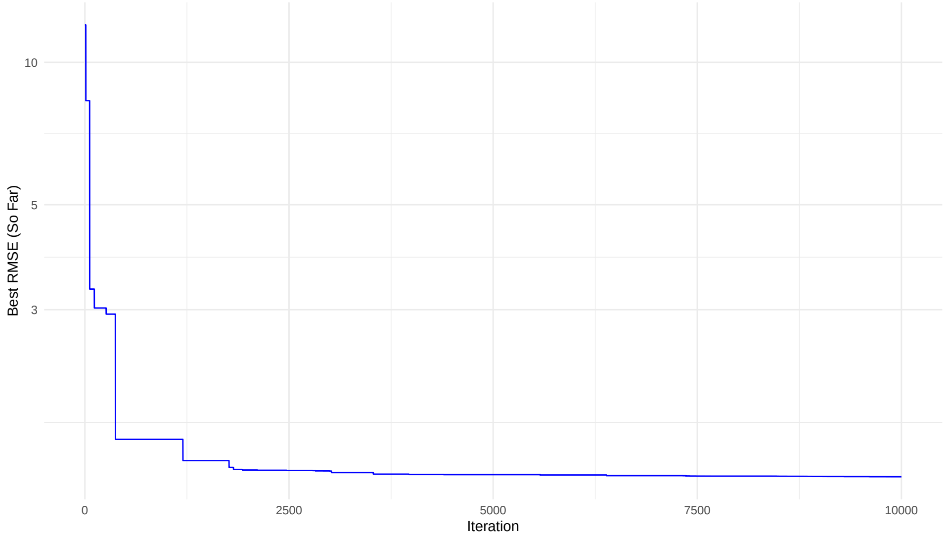
Best RMSE Convergence: Location bigcreek Fold 1
