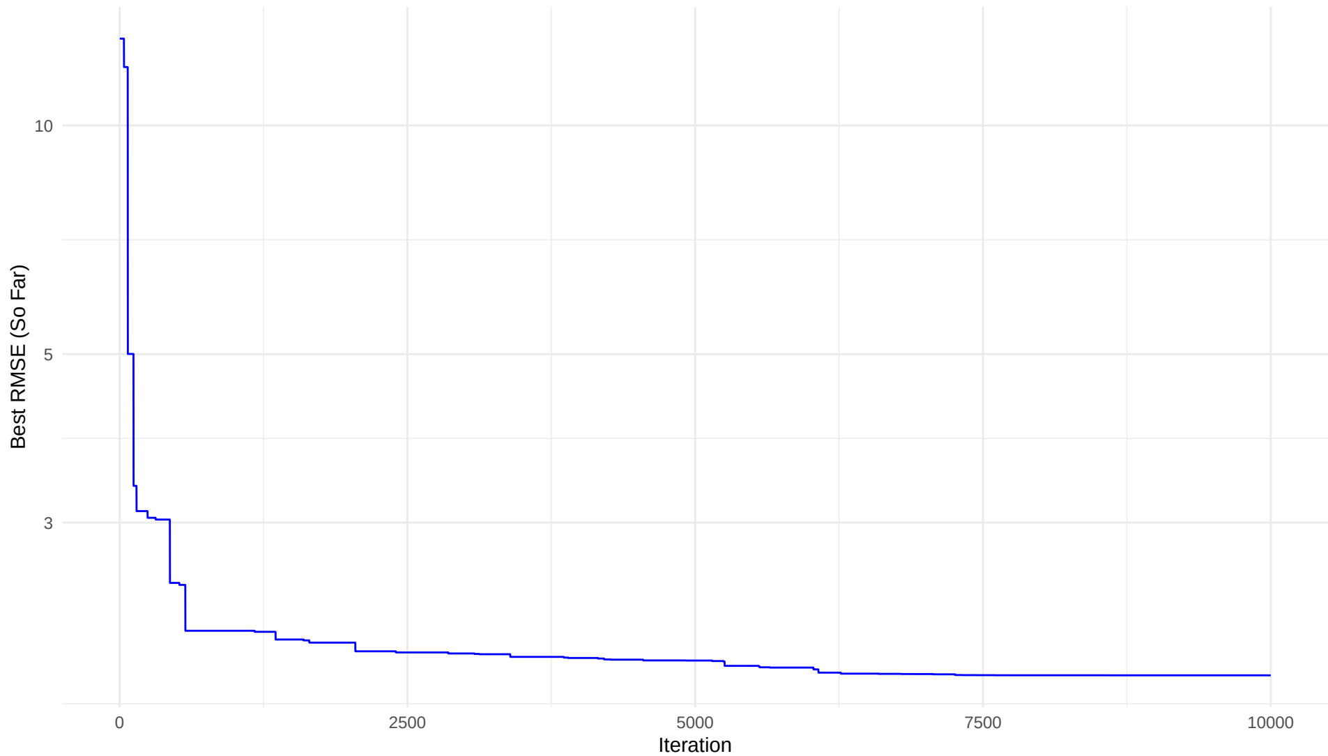
Best RMSE Convergence: Location saginaw Fold 3
