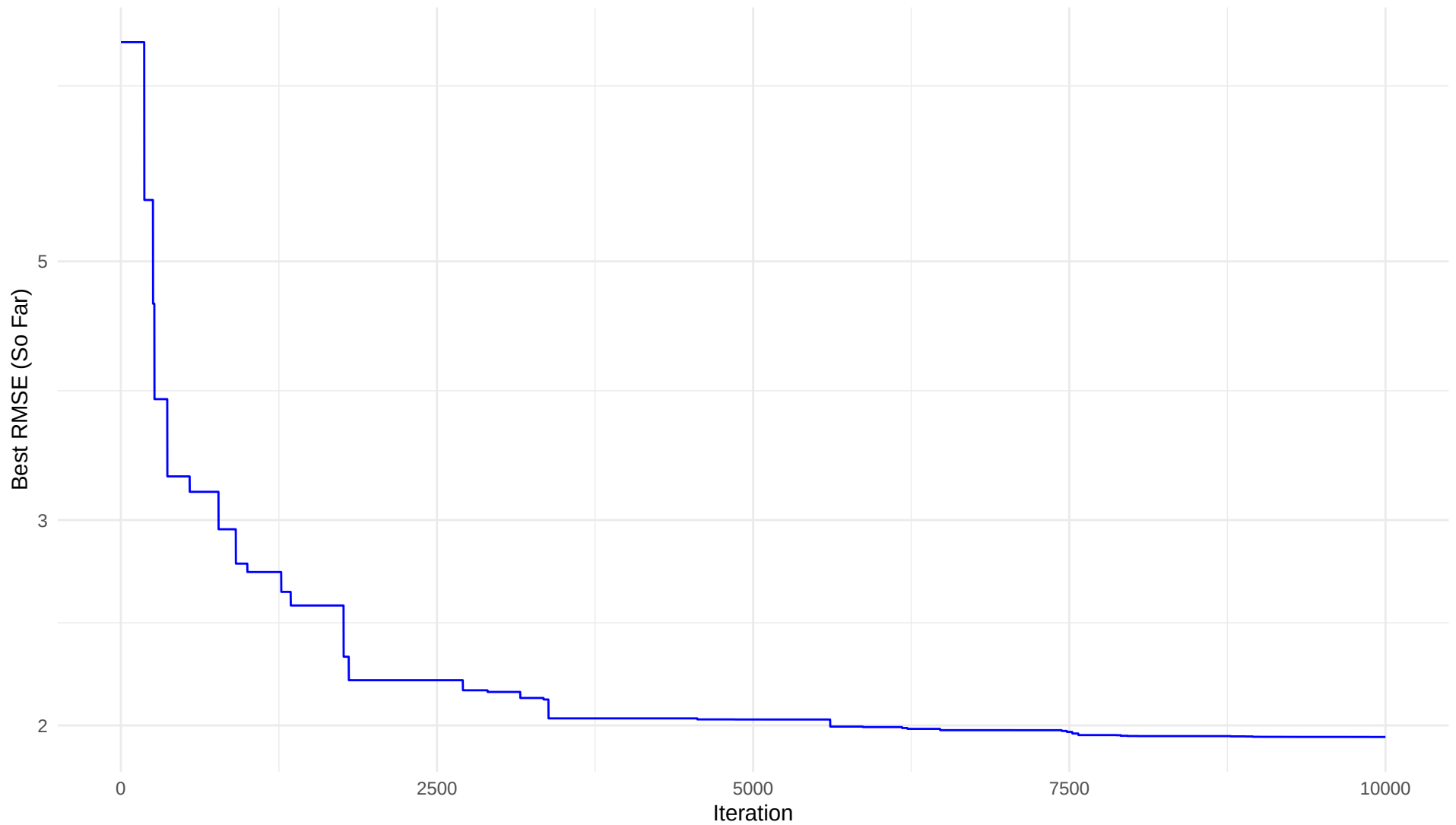
Best RMSE Convergence: Location allegheny Fold 5
