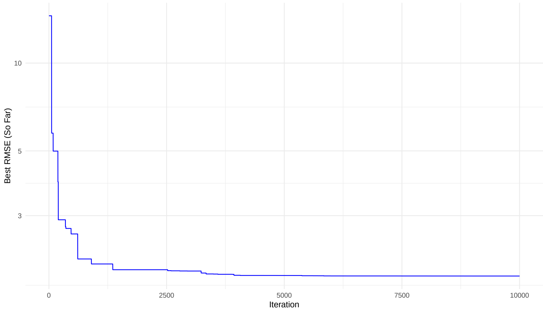
Best RMSE Convergence: Location geneesee Fold 5
